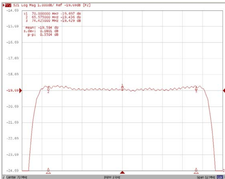
Ripple Variation F_o \pm 4.425\text{MHz}
