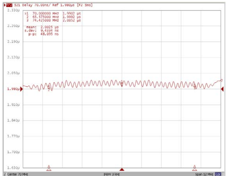
Group Delay Variation F_o \pm 4.425\text{MHz}
